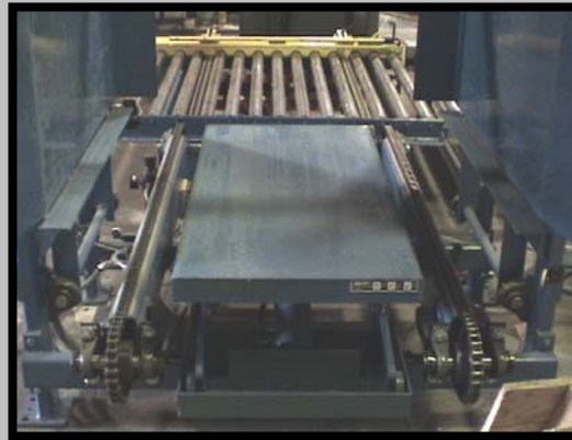
Pallet raising and lowering system
